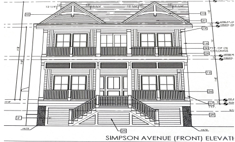
SIMPSON AVENUE (FRONT) ELEVATION
