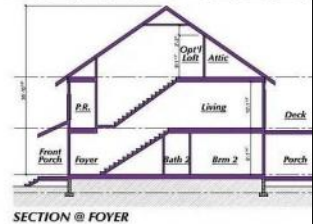
SECTION @ FOYER
